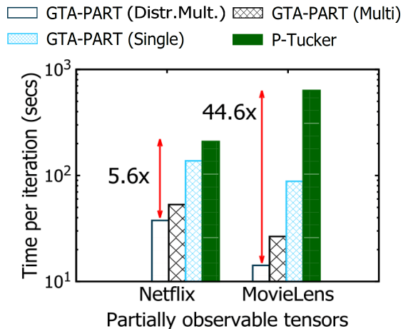
Fig. 6: Performance of GTA-PART and P-TUCKER for real-world partially observable tensors. Distributed-GPU version of GTA-PART shows the fastest factorization speed, which is up to 44.6\times faster than P-TUCKER.
