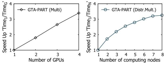
Fig. 9: The GPU scalability of GTA-PART with respect to the number of GPUs (left) and computing nodes (right) used for experiments. GTA-PART presents near-linear scalability regarding the number of GPUs and computing nodes.
